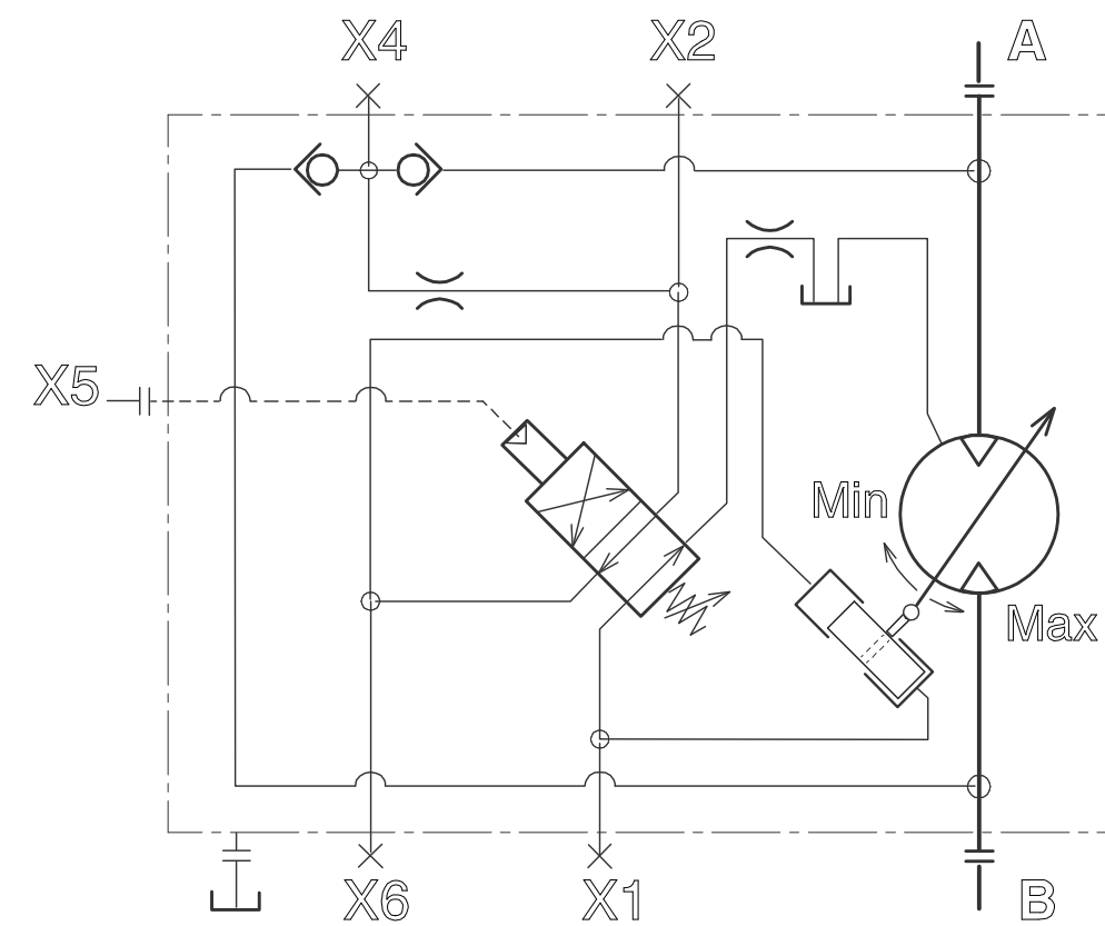
HO S 01 I schematic (X5 not pressurized).
