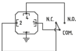
PRESSURE SWITCH
