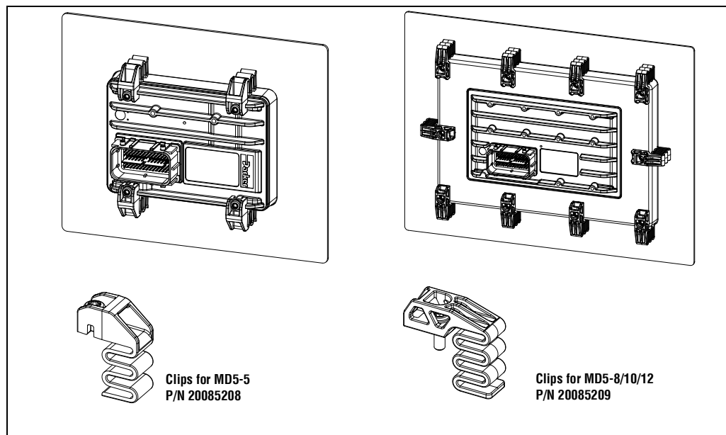
Panel mount with clips for IQAN-MD5
