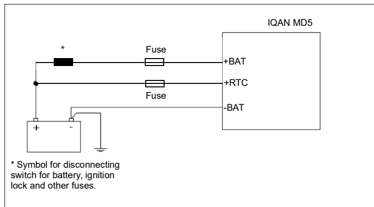
Connecting the RTC and voltage supply.
