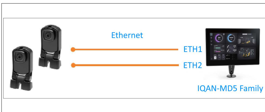
2 x IQAN-SV camera in a system
